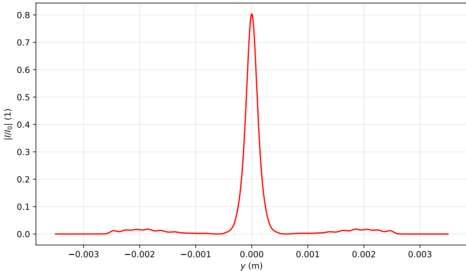
Intensity profile I(x=0, y, z=1.592)/I_0 , \text{Pin}=7.0\text{Pcr} , artificial time
